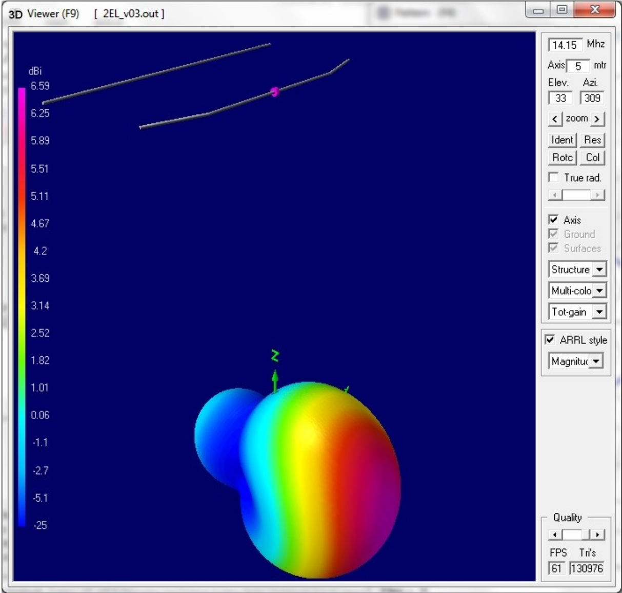
Rob's simulation in 4nec2
